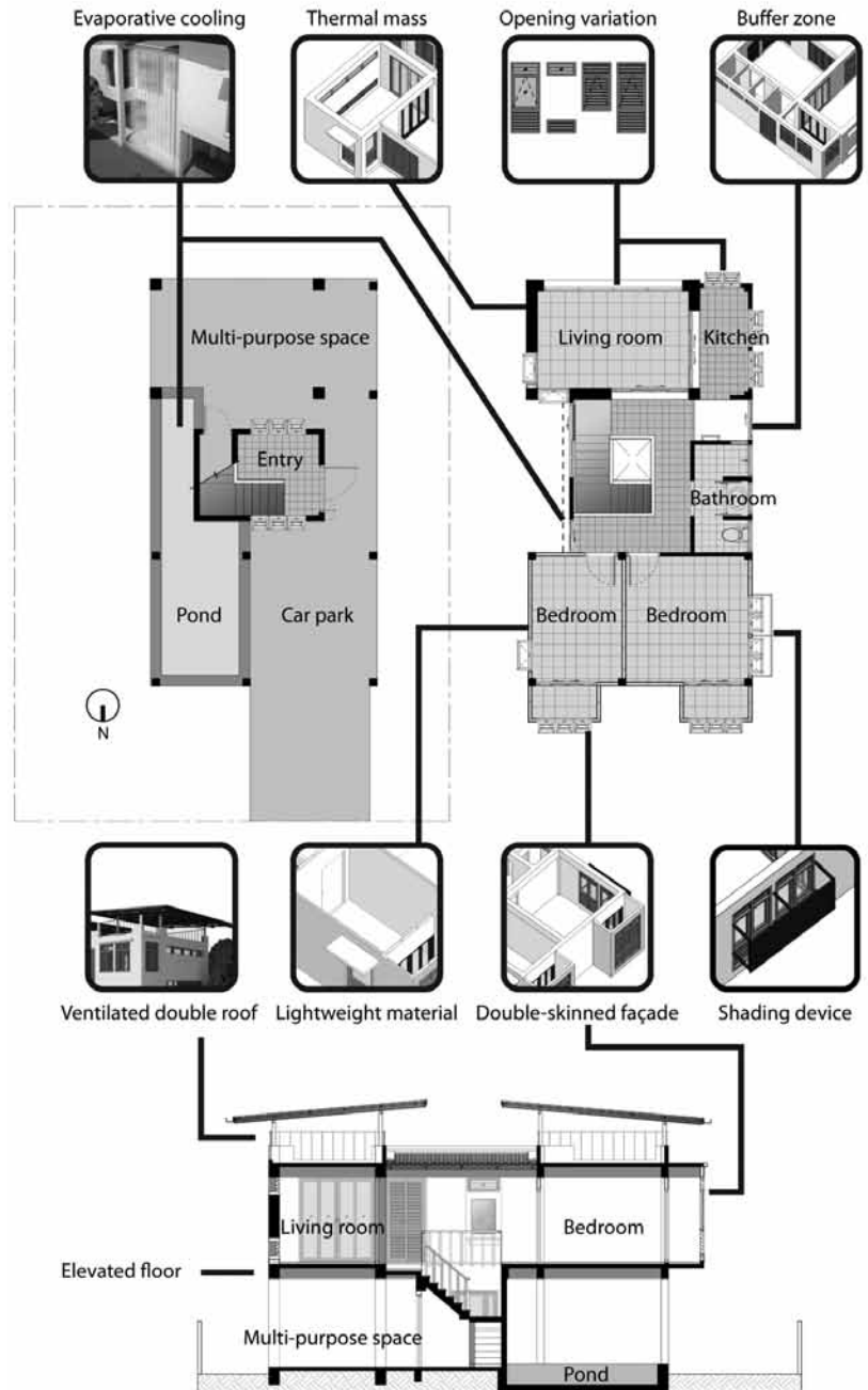
Figure 9. First and second floor plans and longitudinal section of the prototype house showing major design features.
