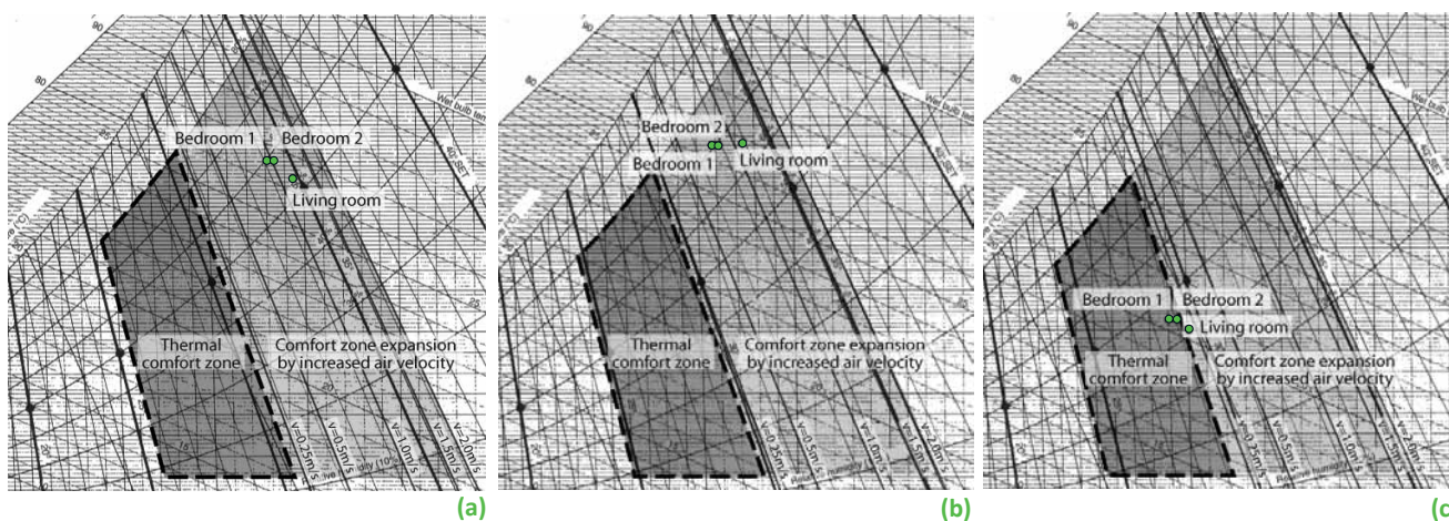
Figure 13. Indoor air conditions of major rooms in (a) April, (b) August, and (c) December as simulated by PasCal (v.1.0).
