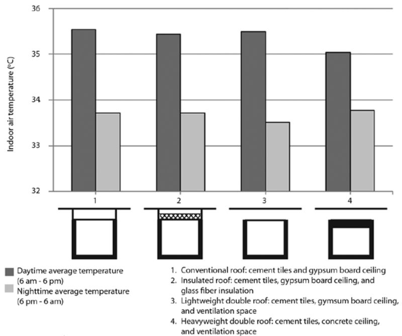
Figure 10. Indoor air temperatures as a result of different roof types as simulated by PasCal (v.1.0).
