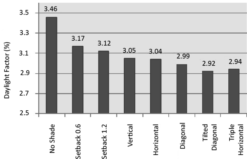
Figure 12. Average daylight factor in an office space of different shading devices.
